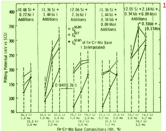
FIGURE 2 — Critical pitting potentials of levitation melted alloys in deaerated synthetic seawater at 90 C, pH = 7.2 ± 0.2.
