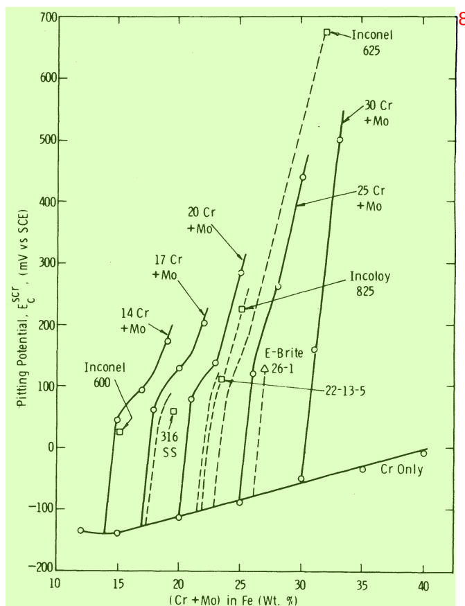
FIGURE 1 — Comparison of the critical pitting potentials of Fe-Cr-Mo alloys with several commercial alloys in deaerated synthetic seawater at 90 C, pH = 7.2 ± 0.2.
