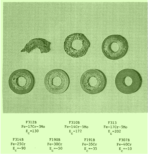
FIGURE 10 — Crevice corrosion after 6 day exposure to oxygenated 10% ferric chloride at 21 ± 1 C. Specimen size: 1/2 inch diameter.
