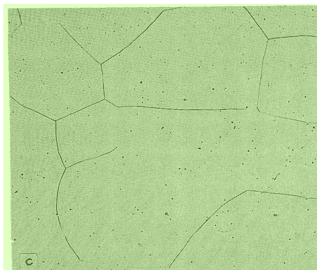
FIGURE 19 — Microstructures of experimental ferritic stainless steel alloys. Left column: transverse 7 to rolling direction; right column: parallel to rolling plane. Electrolytic etch: 10% oxalic acid. (a) Alloy W802, as cold rolled, (b) alloy W882, as cold rolled + 427 C/1 hour, and (c) alloy W849, as cold rolled + 1093 C/1 hour.41X
