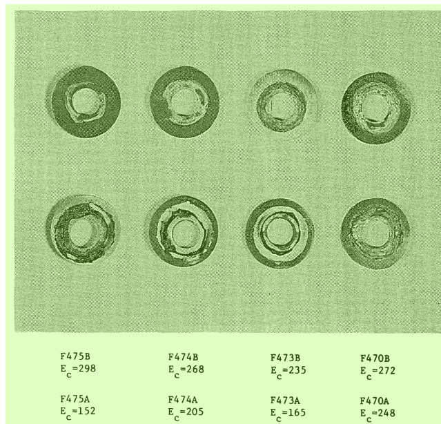
FIGURE 8 — Crevice corrosion after 6 day exposure to oxygenated 10% ferric chloride at 21 ± 1 C. Specimen size: 1/2 inch diameter.
