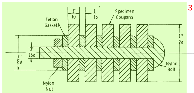
FIGURE 6 — Experimental arrangement of specimens in crevice attack studies.
