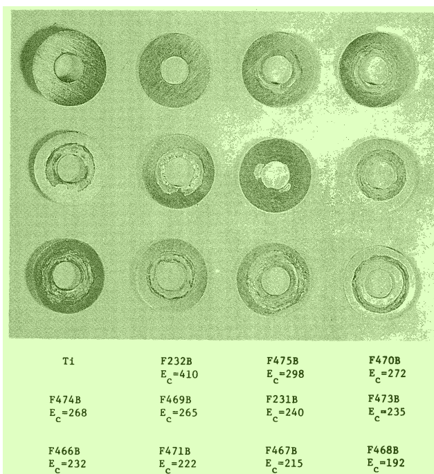
FIGURE 7 — Crevice corrosion after 6 day exposure to oxygenated 10% ferric chloride at 21 ± 1 C. Specimen size: 1/2 inch diameter.
