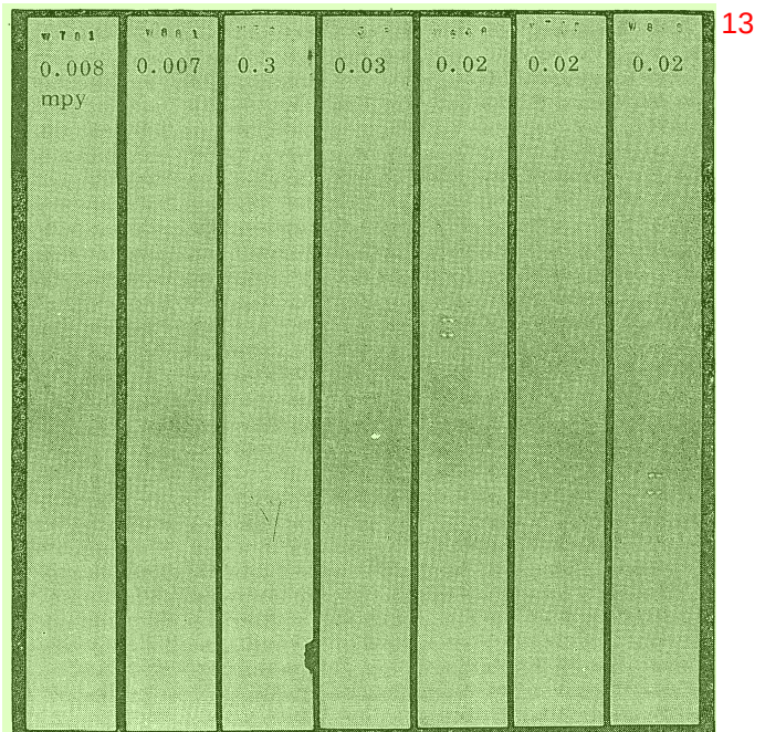
FIGURE 15 – Test coupons of alloys W5, W6, W7, W8, and E-Brite 26-1 (corrosion products removed) after 30 day exposure in Freeport desalination plant at 121 C, 4 ft/sec flow velocity, < 5 ppb dissolved oxygen, < 3 ppm CO 2 , and pH = 7.0 ± 0.1. Initial surface finish pickled 5 minutes at 85 C in 10% HNO 3 -0.5% HF. Note crevice attack on E-Brite 26-1 only.
