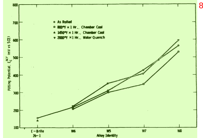
FIGURE 3 — Critical pitting potentials of specimens prepared identically to those used in the desalination plant tests. Measurements made in deaerated synthetic seawater at 90 C, pH = 7.2 ± 0.2.
