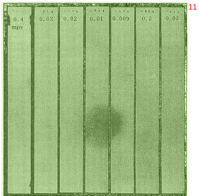
FIGURE 14 – Test coupons of alloys W5, W6, W7, W8, and E-Brite 26-1 (corrosion products removed) after 30 day exposure in Freeport desalination plant at 121 C, 4 ft/sec flow velocity, < 5 ppb dissolved oxygen, < 3 ppm CO 2 , and pH = 7.0 ± 0.1. Initial surface finish pickled 5 minutes at 85 C in 10% HNO 3 -0.5% HF. Note crevice attack on E-Brite 26-1 only.
