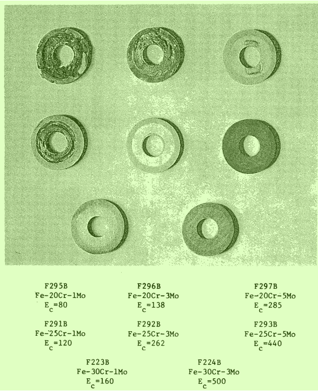
FIGURE 9 — Crevice corrosion after 6 day exposure to oxygenated 10% ferric chloride at 21 ± 1 C. Specimen size: 1/2 inch diameter.
