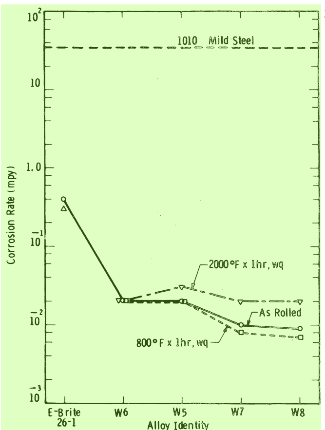
FIGURE 4 — Corrosion rates after Run 1 in desalination plant.
