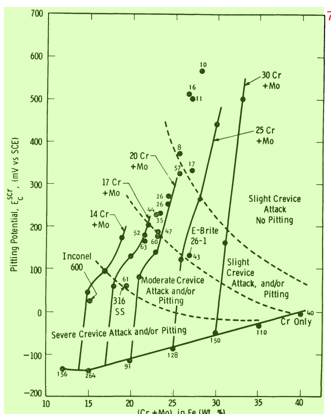
FIGURE 22 — Relationship between the critical pitting potentials ( E_c^{scr} measured in deaerated synthetic seawater at 90 C, pH = 7.2 \pm 0.2) of Fe-Cr-Mo based alloys and their resistance to crevice attack after a 14 day exposure to synthetic seawater at 121 C and \sim 60 ppm oxygen. The numbers associated with individual points indicate the weight losses expressed as gms \times 10^{-4} after the 121 C exposure for samples with initial weights of \sim 1 gm.
