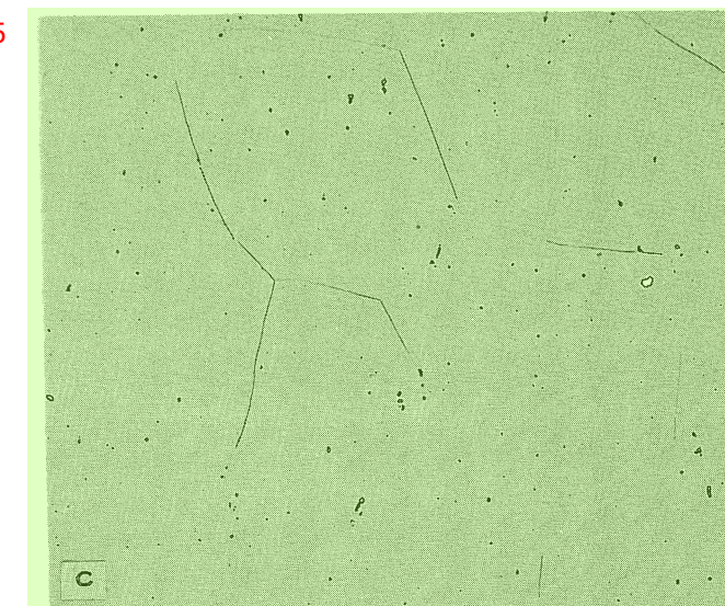
FIGURE 19 — Microstructures of experimental ferritic stainless steel alloys. Left column: transverse 7 to rolling direction; right column: parallel to rolling plane. Electrolytic etch: 10% oxalic acid. (a) Alloy W802, as cold rolled, (b) alloy W882, as cold rolled + 427 C/1 hour, and (c) alloy W849, as cold rolled + 1093 C/1 hour.41X
