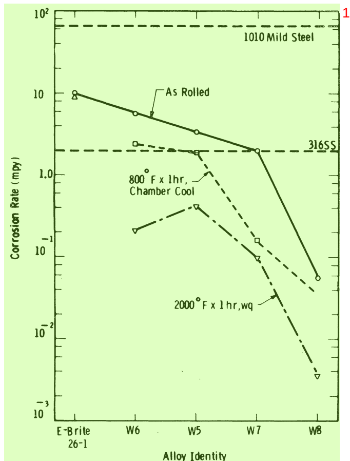
FIGURE 5 — Corrosion rates after Run 5 in desalination plant.
